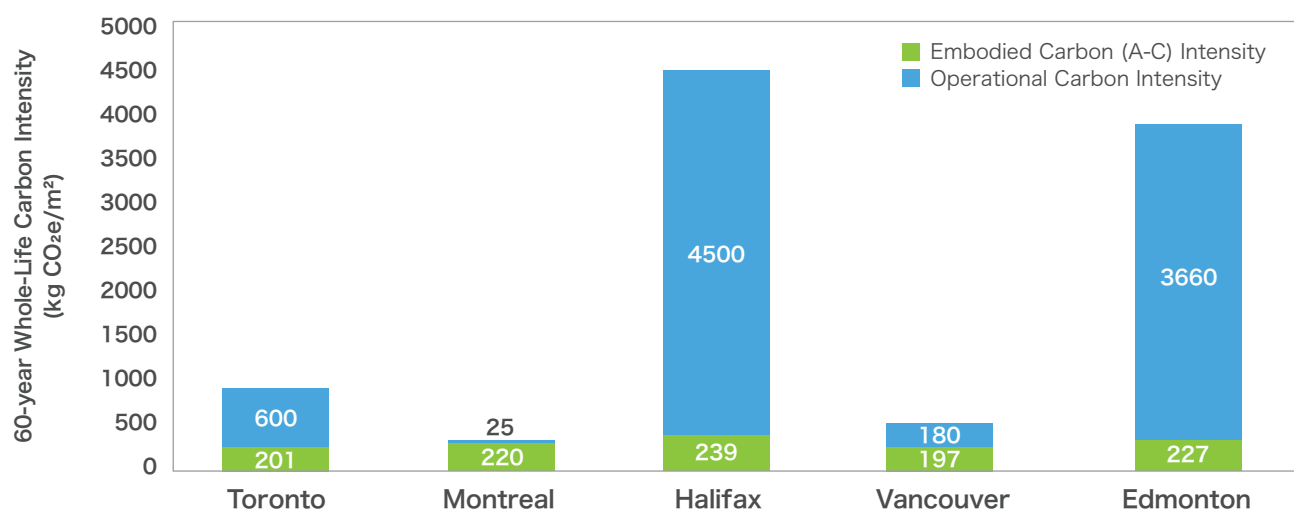
Figure 7: Whole-life carbon intensity (A-C), with breakdowns of embodied and operational carbon intensity, over 60 years. Green represents embodied carbon intensity, and blue represents operation carbon intensity. Operational carbon emissions vary across regions due to differences in climate (energy demand), energy efficiency requirements, and the emission intensity of local energy systems (including the electricity grid).
